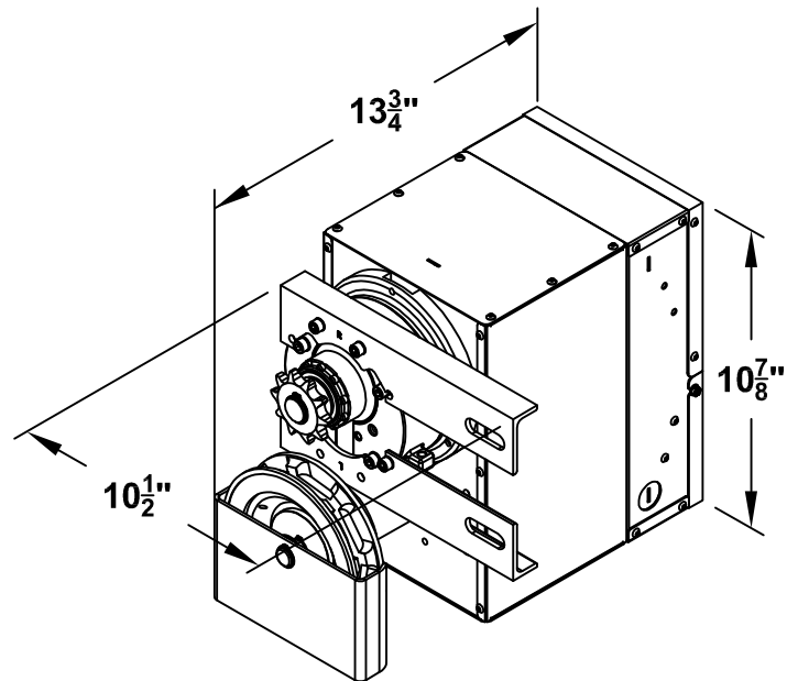
CHAIN OPERATION (FD-2A)
