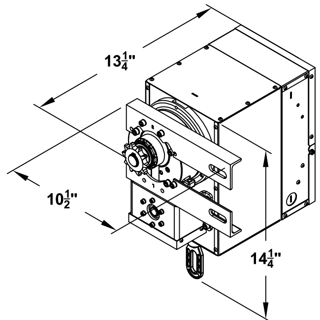
CRANK OPERATION (FD-3A)
