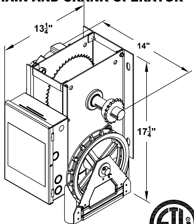
CHAIN OPERATION
