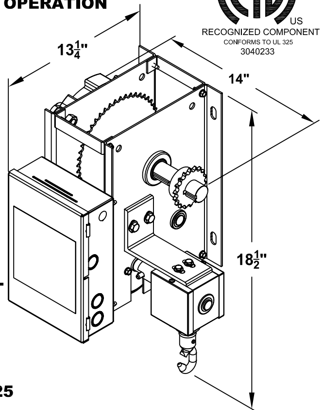
CRANK OPERATION
