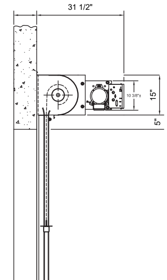
Standard AlarmGard® Motor Operator Side View
