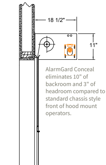
AlarmGard® Conceal Side View
