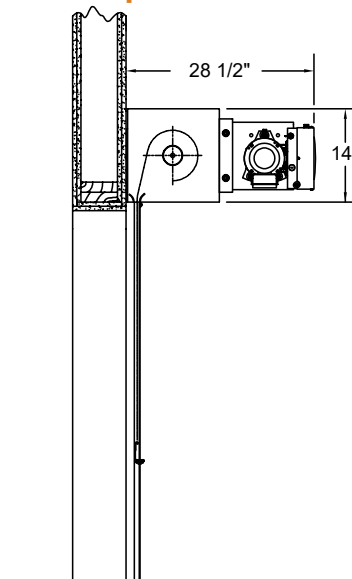
Standard AlarmGard® Motor Operator Side View
